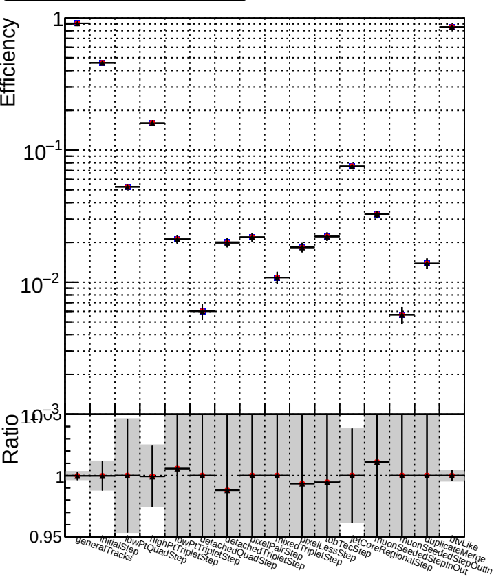
DQM_TT_mkFit-DQM_old132 DQM_TT_mkFit-DQM_new132 DQM_TT_mkFit-DQM_newfast132
