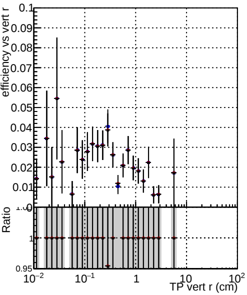
Efficiency vs TP vert r (cm) Legend: DQM_TT_mkFit-DQM_old132 DQM_TT_mkFit-DQM_new132 DQM_TT_mkFit-DQM_newfast132
