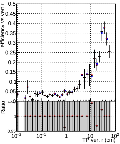
Efficiency vs TP vert r (cm) DQM_TT_mkFit-DQM_old132 DQM_TT_mkFit-DQM_new132 DQM_TT_mkFit-DQM_newfast132
