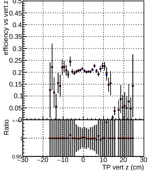
Efficiency vs vert z —●— DQM_TT_mkFit-DQM_old132 —●— DQM_TT_mkFit-DQM_new132 —●— DQM_TT_mkFit-DQM_newfast132
