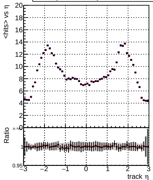
mean hits — DQM_TT_mkFit-DQM_old132 — DQM_TT_mkFit-DQM_new132 — DQM_TT_mkFit-DQM_newfast132
