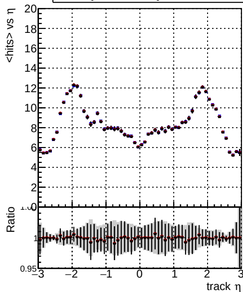
mean hits DQM_TT_mkFit-DQM_old132 DQM_TT_mkFit-DQM_new132 DQM_TT_mkFit-DQM_newfast132
