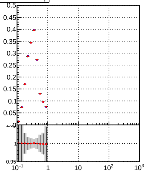
DQM_TT_mkFit-DQM_orig2 DQM_TT_mkFit-DQM_mod2
