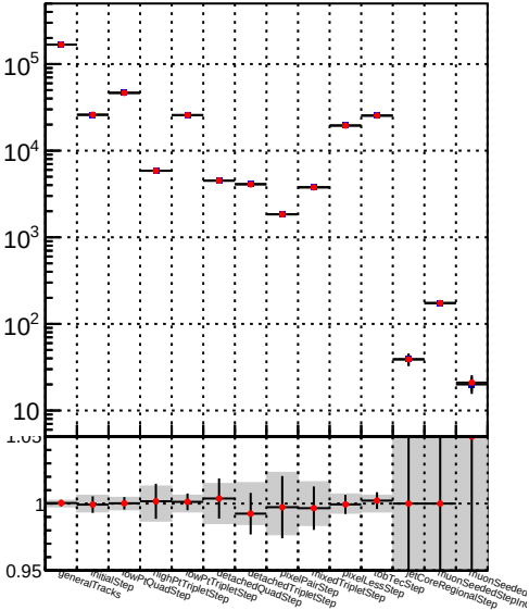
Number —●— DQM_TT__mkFit-DQM_mod2
