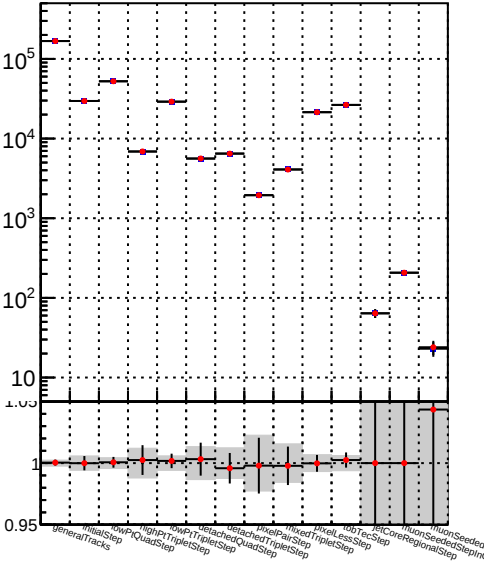
Number —●— DQM_TT__mkFit-DQM_mod2
