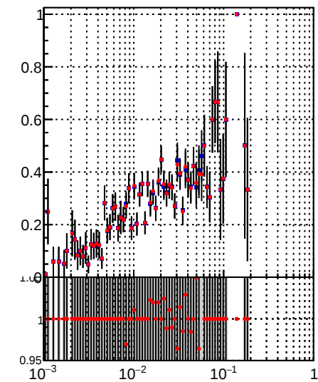
—•— DQM_TT_mkFit-DQM_orig2 —•— DQM_TT_mkFit-DQM_mod2
