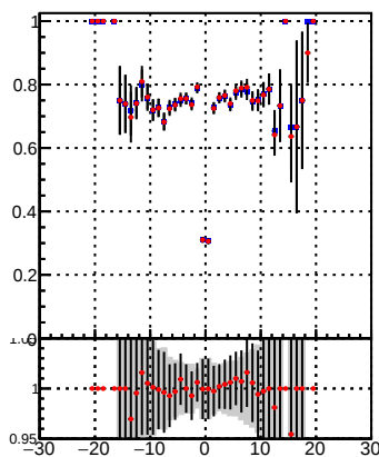
Pileup rate vs dzpvp
