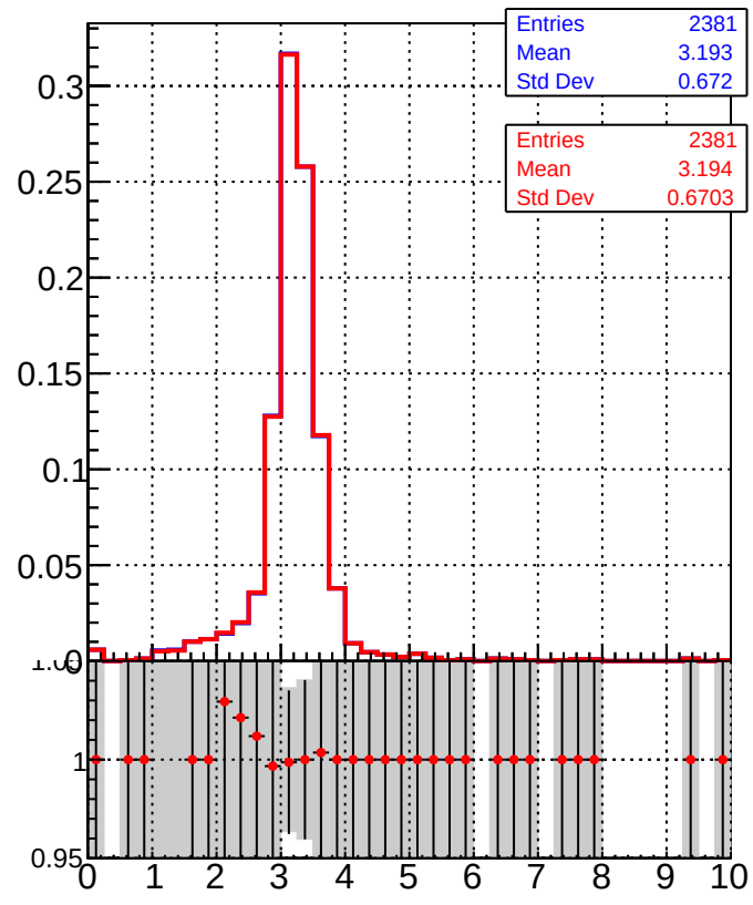
Legend: DQM_TT_mkFit-DQM_orig2 DQM_TT_mkFit-DQM_mod2
