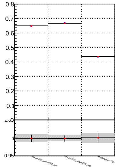
Fake rate vs. — DQM_TT_mkFit-DQM_orig2 — DQM_TT_mkFit-DQM_mod2
