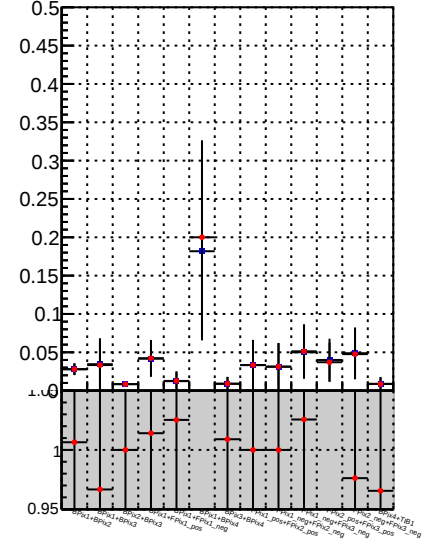
Fake rate vs. — DQM_TT_mkFit-DQM_orig2 — DQM_TT_mkFit-DQM_mod2
