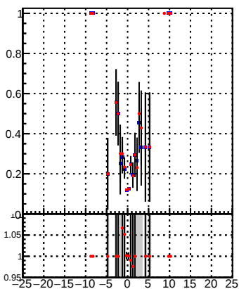
—•— DQM_TT_mkFit-DQM_orig2 —•— DQM_TT_mkFit-DQM_mod2
