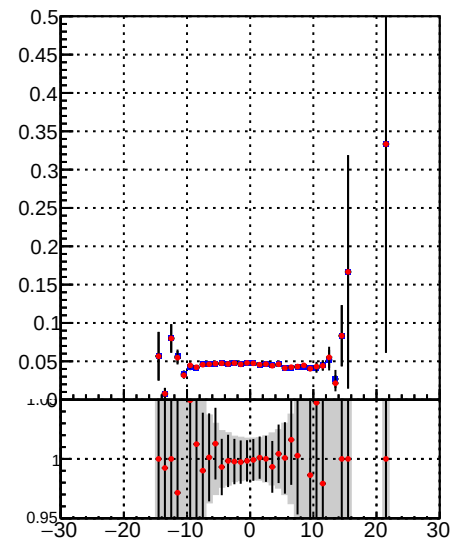
Fake rate vs d
