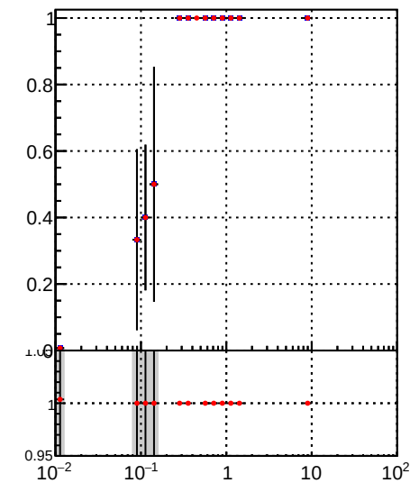
■ DQM_TT_mkFit-DQM_orig2 ● DQM_TT_mkFit-DQM_mod2
