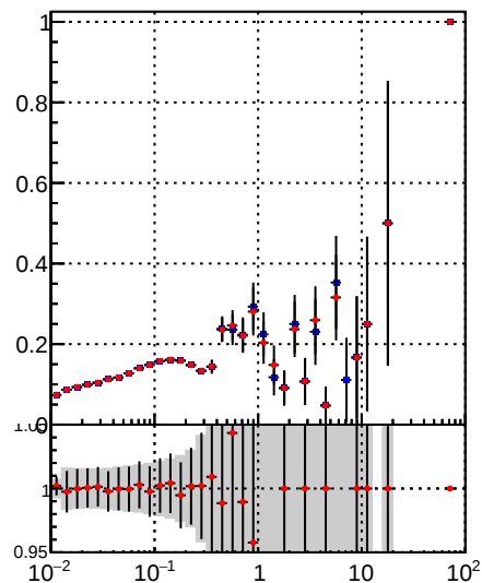
—•— DQM_TT_mkFit-DQM_orig2 —•— DQM_TT_mkFit-DQM_mod2
