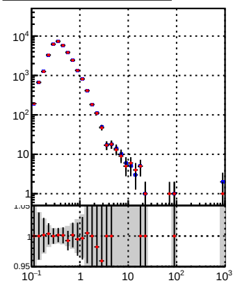
—●— DQM_TT_mkFit-DQM_orig2 —●— DQM_TT_mkFit-DQM_mod2
