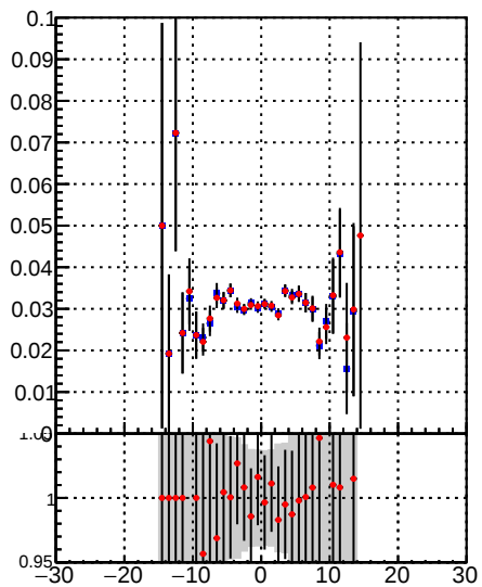
Fake rate vs d —●— DQM_TT_mkFit-DQM_orig2 —●— DQM_TT_mkFit-DQM_mod2
