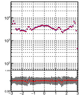
N of reco track vs \eta pT 800 Legend: DQM_TT_mkFit-DQM_orig2 (blue line with dots) DQM_TT_mkFit-DQM_mod2 (red line with dots)
