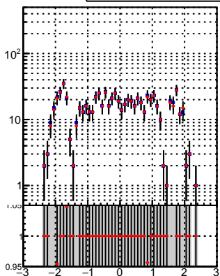
—●— DQM_TT_mkFit-DQM_orig2 —●— DQM_TT_mkFit-DQM_mod2
