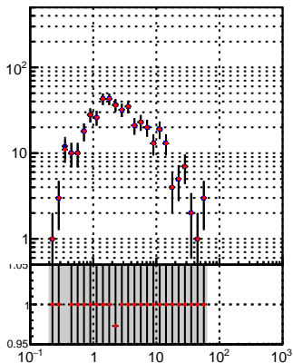
—●— DQM_TT_mkFit-DQM_orig2 —●— DQM_TT_mkFit-DQM_mod2
