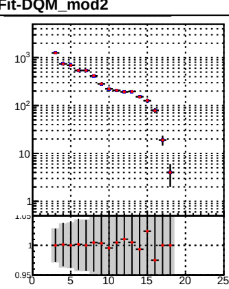
DQM_TT_mkFit-DQM_orig2 DQM_TT_mkFit-DQM_mod2
