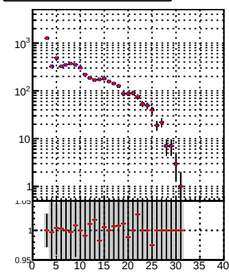
DQM_TT_mkFit-DQM_orig2 DQM_TT_mkFit-DQM_mod2
