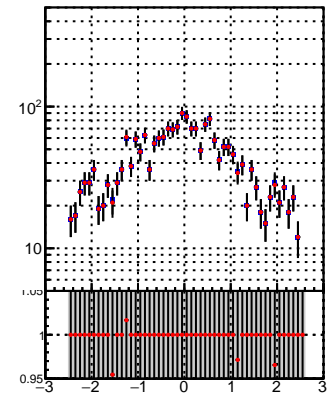
N of reco track vs \phi vs eta Legend: DQM_TT_mkFit-DQM_orig2 (blue line with markers) DQM_TT_mkFit-DQM_mod2 (red line with markers)
