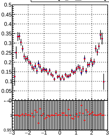
—•— DQM_TT_mkFit-DQM_orig2 —•— DQM_TT_mkFit-DQM_mod2
