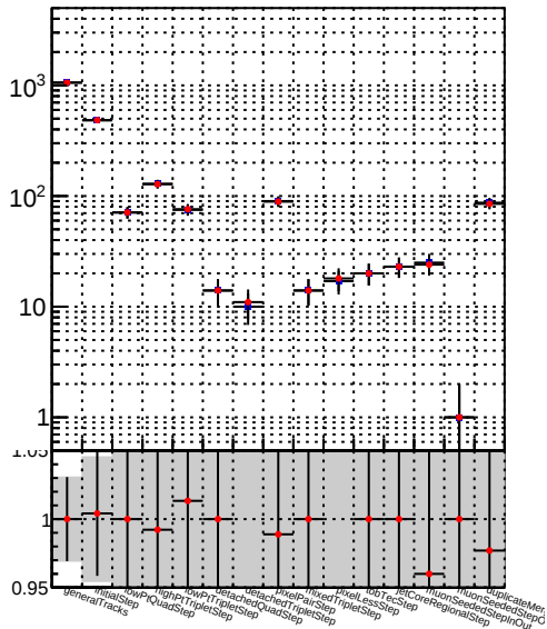
Number —●— DQM_TT__mkFit-DQM_mod2
