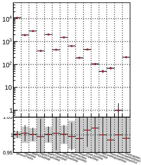
Number —●— DQM_TT__mkFit-DQM_mod2
