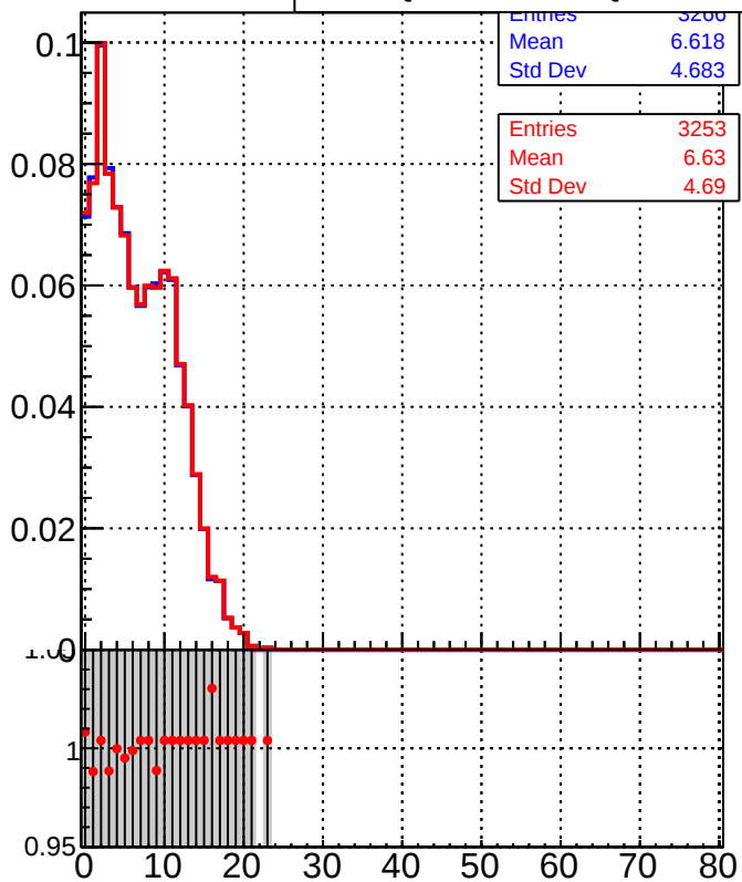
Legend: DQM_TT_mkFit-DQM_orig2 (grey histogram, blue line with points), DQM_TT_mkFit-DQM_mod2 (red line with points)
