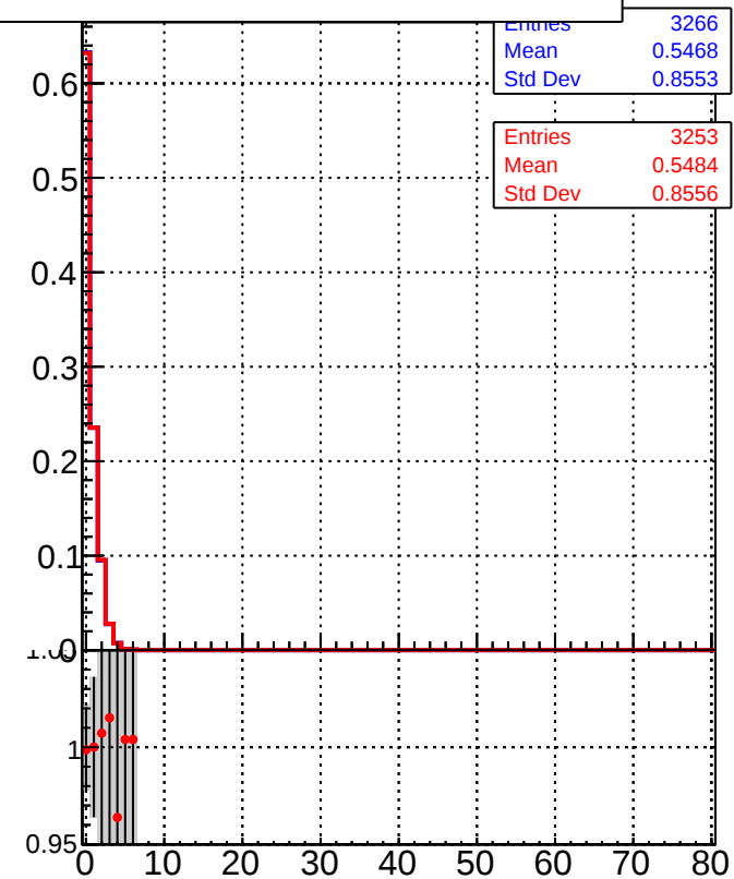
Legend: DQM_TT_mkFit-DQM_orig2 (grey histogram, blue line with points), DQM_TT_mkFit-DQM_mod2 (red line with points)
