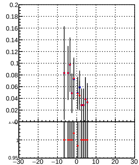
Fake rate vs d —●— DQM_TT_mkFit-DQM_orig2 —●— DQM_TT_mkFit-DQM_mod2
