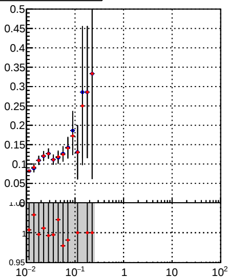
—•— DQM_TT_mkFit-DQM_orig2 —•— DQM_TT_mkFit-DQM_mod2
