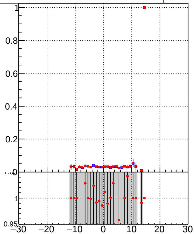
DQM_TT_mkFit-DQM_orig2 DQM_TT_mkFit-DQM_mod2
