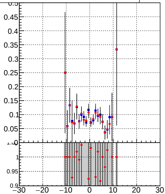
DQM_TT_mkFit-DQM_orig2 DQM_TT_mkFit-DQM_mod2
