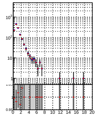
N of reco track vs. \chi^2 —•— mkFit-DQM_orig2 —•— mkFit-DQM_mod2
