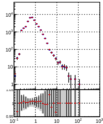
DQM_TT_mkFit-DQM_orig2 DQM_TT_mkFit-DQM_mod2
