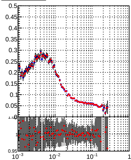
Legend: DQM_TT_mkFit-DQM_orig2 (blue squares) DQM_TT_mkFit-DQM_mod2 (red circles) Fake rate vs dr
