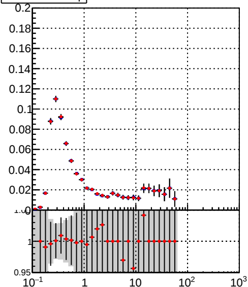
■ DQM_TT_mkFit-DQM_orig2 ■ DQM_TT_mkFit-DQM_mod2
