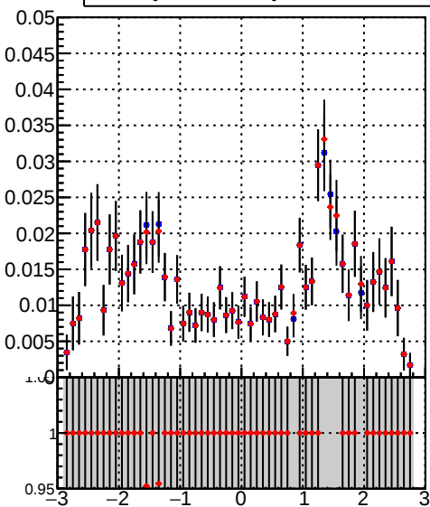
■ DQM_TT_mkFit-DQM_orig2 ■ DQM_TT_mkFit-DQM_mod2
