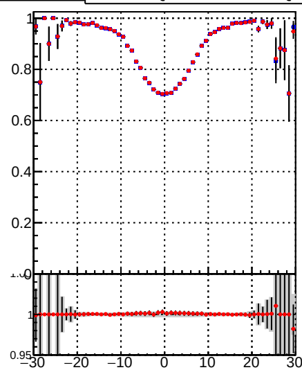
■ DQM_TT_mkFit-DQM_orig2 ■ DQM_TT_mkFit-DQM_mod2
