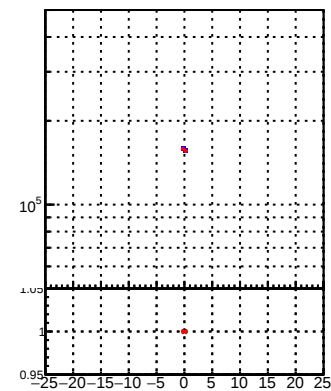
DQM_TT_mkFit-DQM_orig2 DQM_TT_mkFit-DQM_mod2
