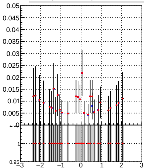
Legend: DQM_TT_mkFit-DQM_orig2 (blue squares), DQM_TT_mkFit-DQM_mod2 (red circles)
