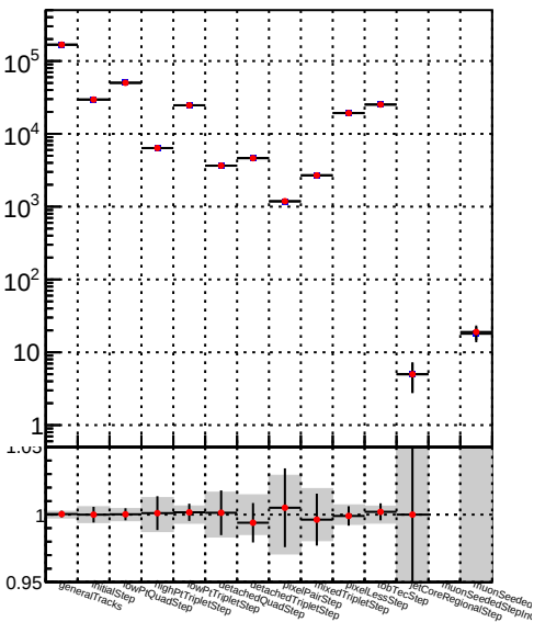
Number —●— DQM_TT__mkFit-DQM_mod2
