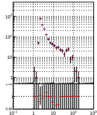
—●— DQM_TT_mkFit-DQM_orig2 —●— DQM_TT_mkFit-DQM_mod2
