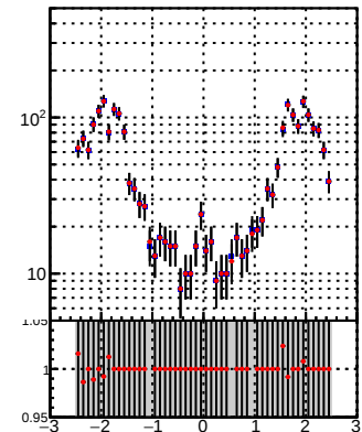
—●— DQM_TT_mkFit-DQM_orig2 —●— DQM_TT_mkFit-DQM_mod2
