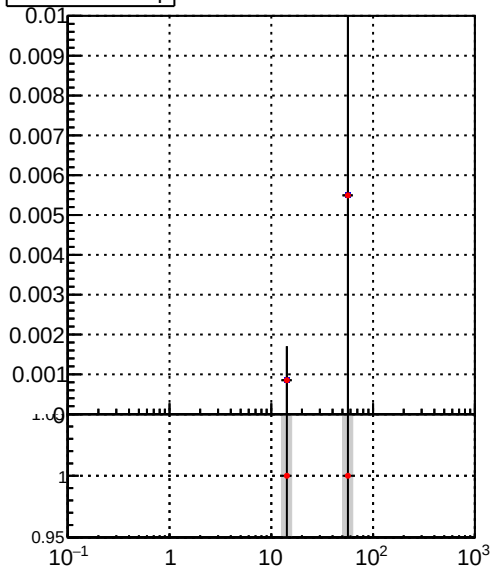
DQM_TT_mkFit-DQM_orig2 DQM_TT_mkFit-DQM_mod2
