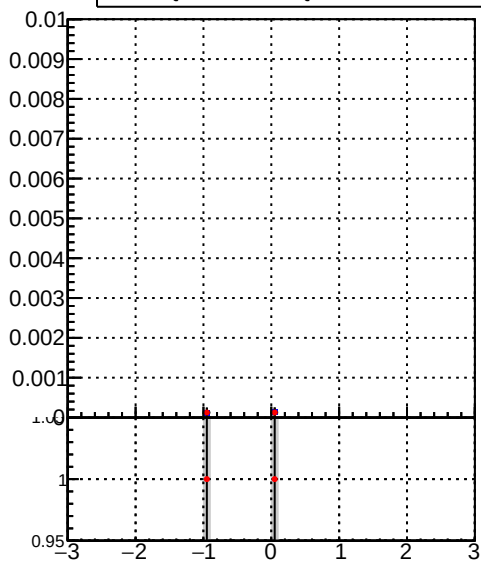
DQM_TT_mkFit-DQM_orig2 DQM_TT_mkFit-DQM_mod2
