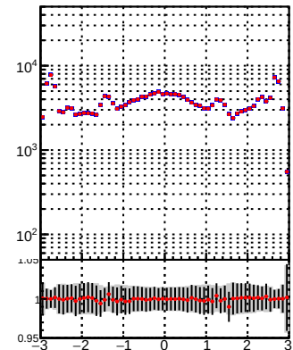
N of reco track vs \eta Legend: —•— DQM_TT_mkFit-DQM_orig2 —•— DQM_TT_mkFit-DQM_mod2
