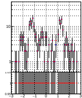
N of reco track vs \eta DQM TT mkFit-DQM_orig2 N of reco track vs \eta DQM TT mkFit-DQM_mod2
