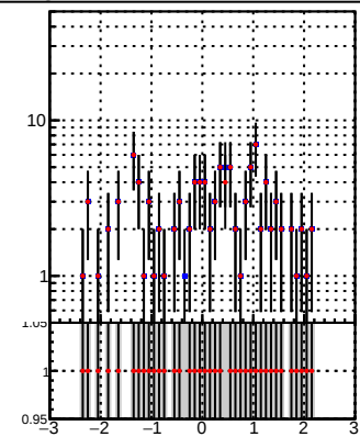
— DQM_TT_mkFit-DQM_orig2 — DQM_TT_mkFit-DQM_mod2
