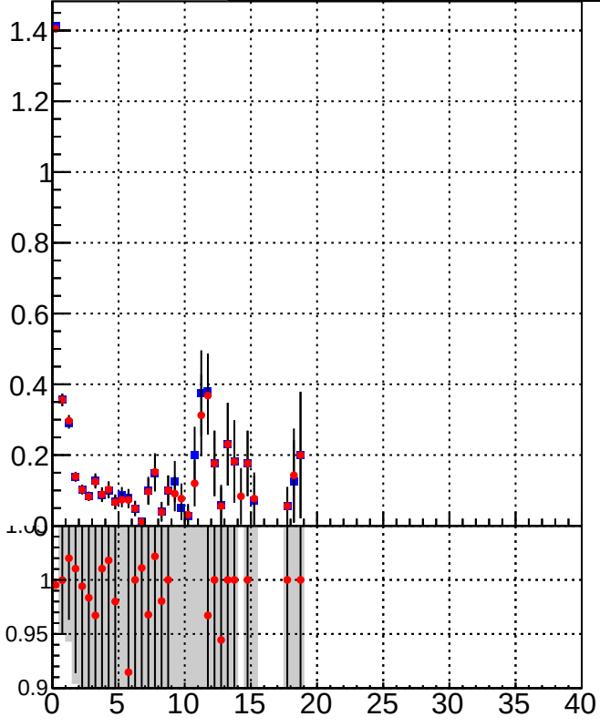
K_S^0 tracking fake rate vs p_T and \eta Legend: DQM_TT_mkFit-DQM_orig2 (blue star) DQM_TT_mkFit-DQM_mod2 (red star)
