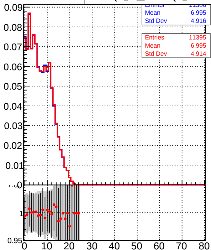
—■— DQM_TT_mkFit-DQM_orig2 —●— DQM_TT_mkFit-DQM_mod2
