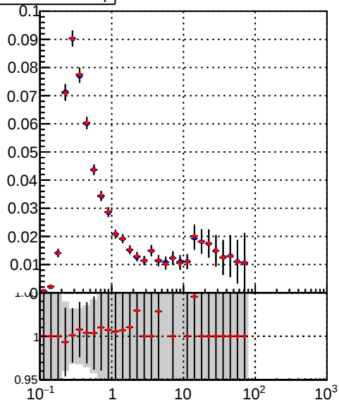
—●— DQM_TT_mkFit-DQM_orig2 —●— DQM_TT_mkFit-DQM_mod2
