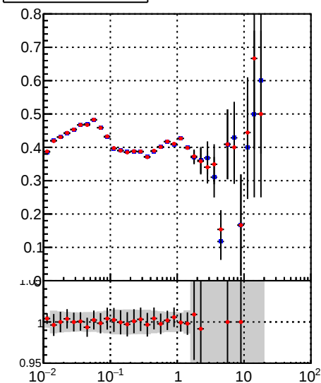
■ DQM_TT_mkFit-DQM_orig2 ● DQM_TT_mkFit-DQM_mod2
