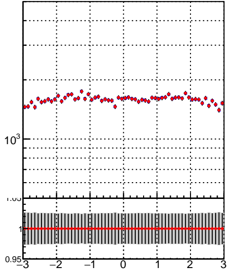
N of simulated tracks vs phi Legend: - DQM_TT_mkFit-DQM_orig (grey histogram) - DQM_TT_mkFit-DQM_mod (red line)
